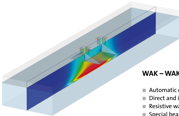
Beam position monitor at v = 0.75c
