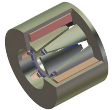
Model of a claw pole induction generator
