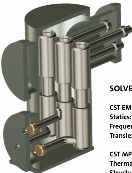
50 Hz gas-insulated switch
